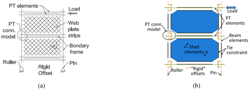
Figure 6. Example of (a) strip model and (b) shell element web plate model for a UW subassembly test.
