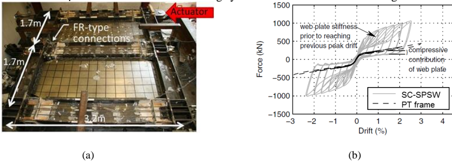
Figure 2. UW Subassembly test (a) test set-up and (b) sample results.
