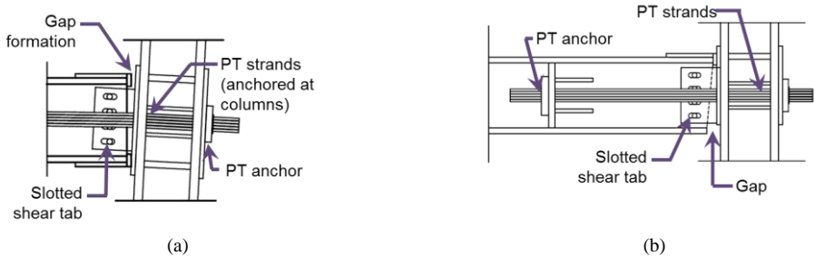
Figure 1. (a) FR and (b) NewZ-BREAKSS PT connections.
